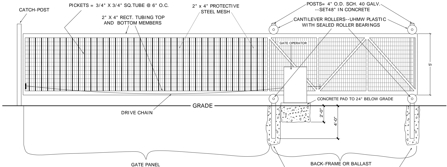
VIEW FROM INSIDE--CLOSED CONDITION
